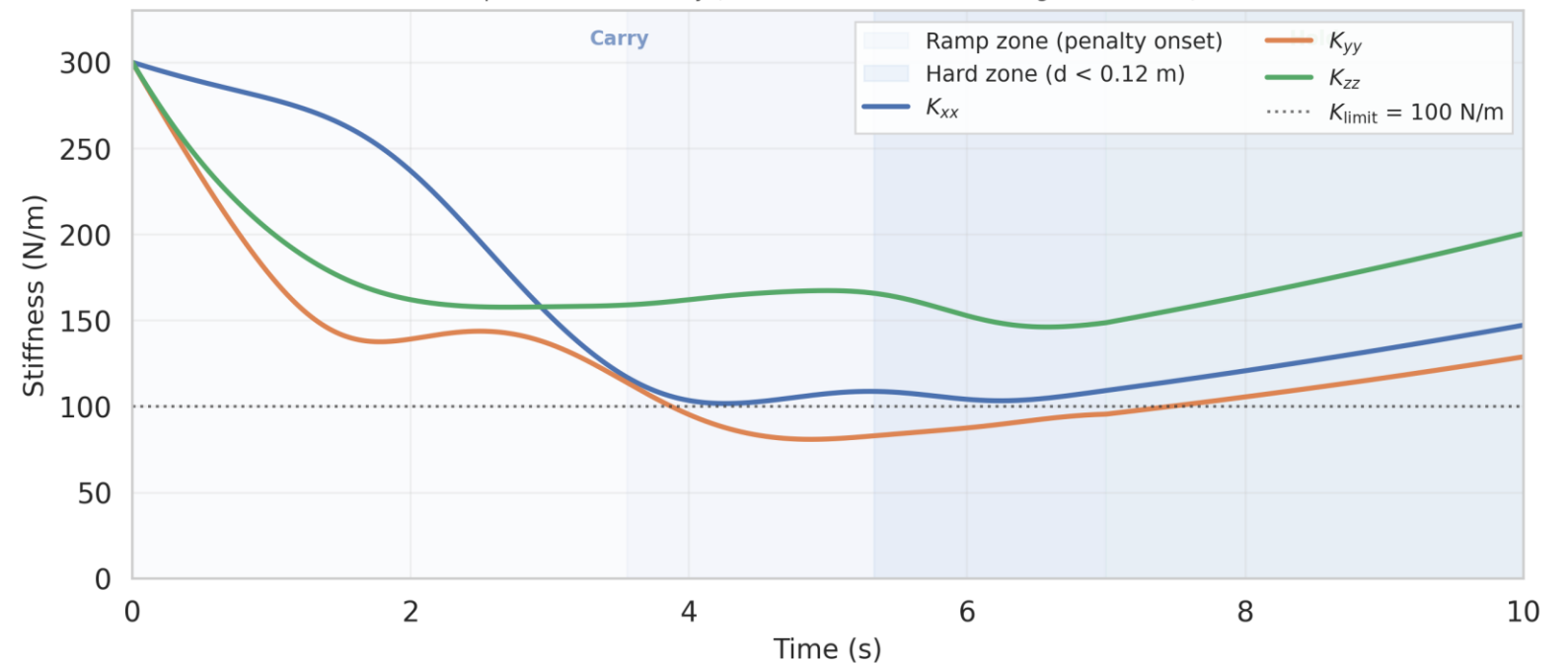
Exp 3b — Ball Delivery (soft obstacle avoidance, weight-controlled)
