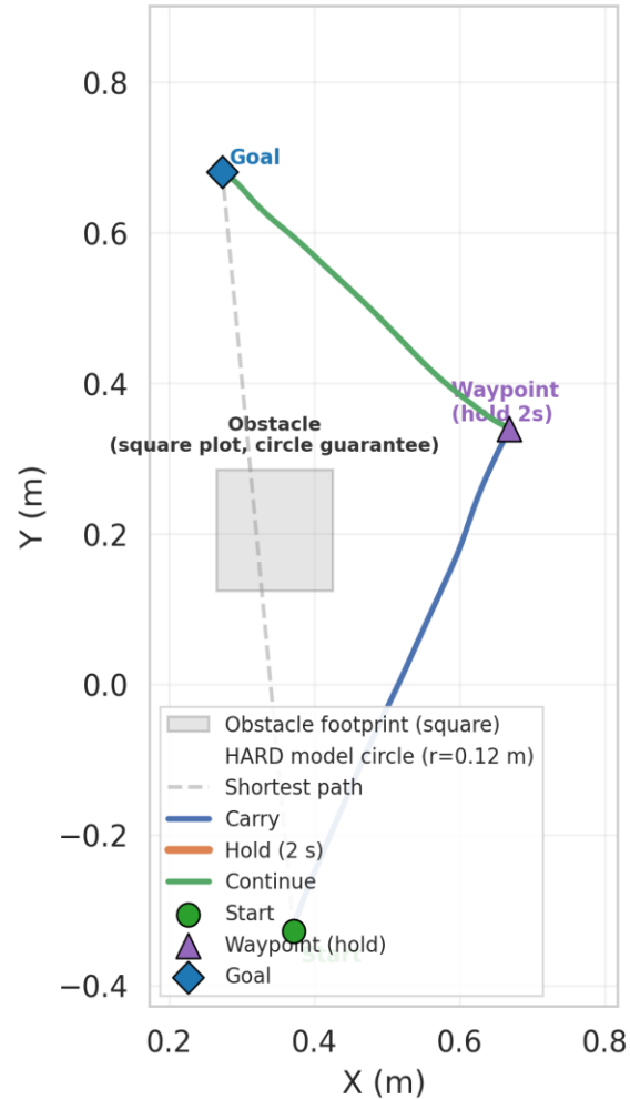
Top-down view (X-Y) Scene 4 — Carry → Hold (2 s) → Continue (HARD obstacle avoidance)
