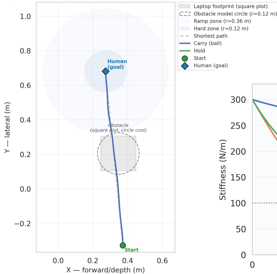
Top-down view: table plane (X-Y) Exp 3b — Ball Delivery (soft obstacle avoidance, weight-controlled)
